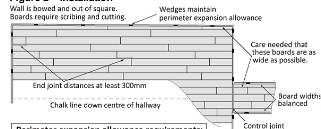
Figure 2 – Installation
